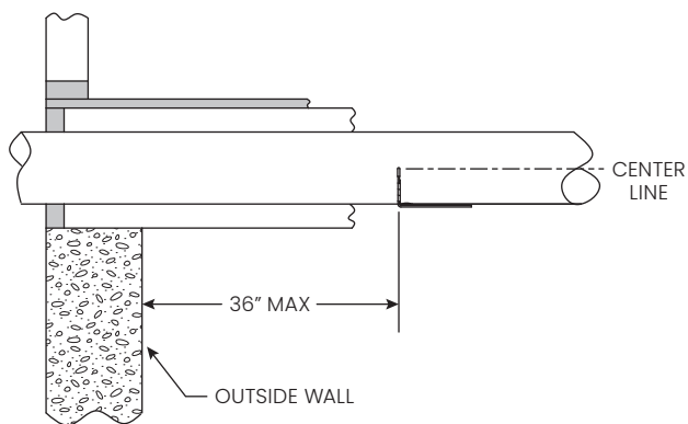
FIGURE 13: ODT MOUNTED IN INTAKE DUCT
