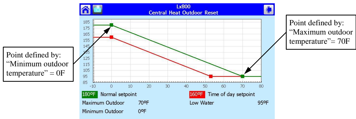
Figure 4-7 Outdoor Reset Line
