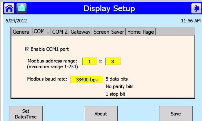
Figure 9-7 COM1 Settings
