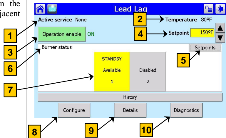
Figure 8-1 Lead Lag Master Screen
