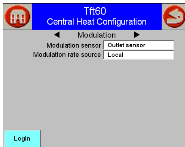
Figure 4-5 Central Heat Configuration – Modulation
