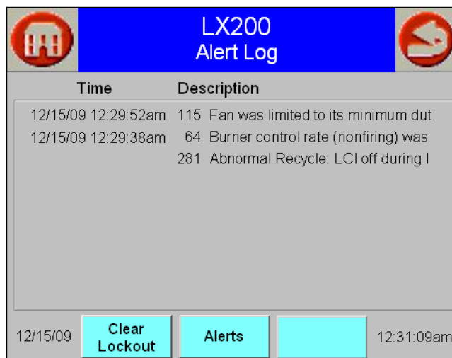
Figure 7-4 Alert Log and Events
